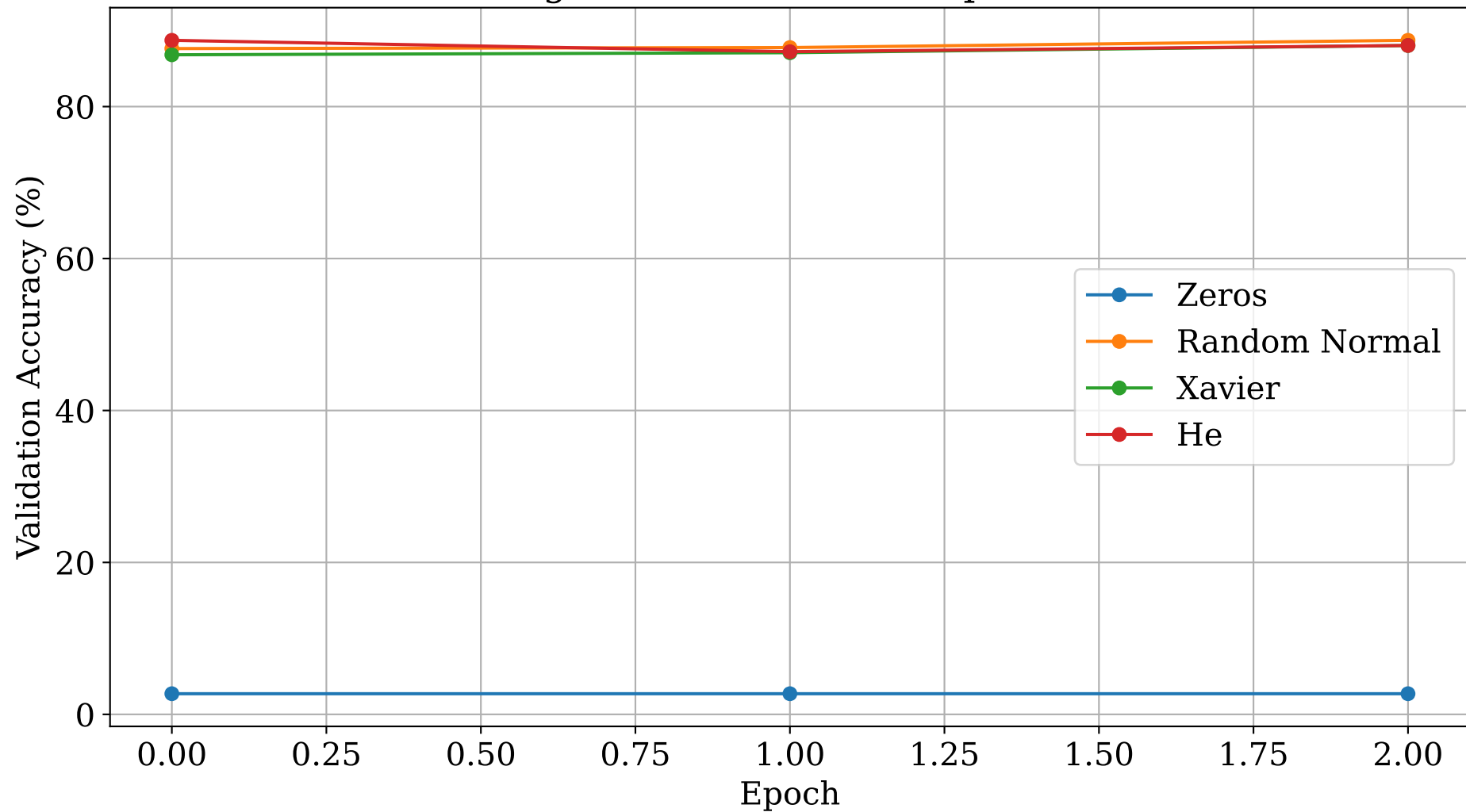
Weight Initialization Comparison
